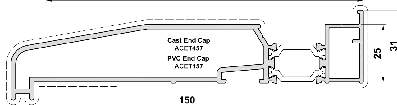
ETC457 150mm Cill
