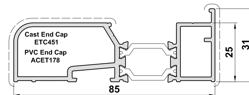
ETC451 85mm Cill
