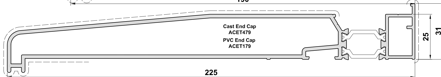
ETC479 225mm Cill
