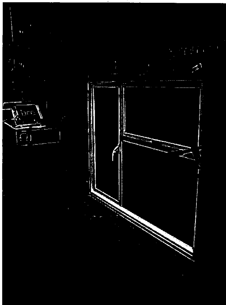
Figure A1. Smart Systems Alitherm 300 casement window in the BRE Test rig 'G'
