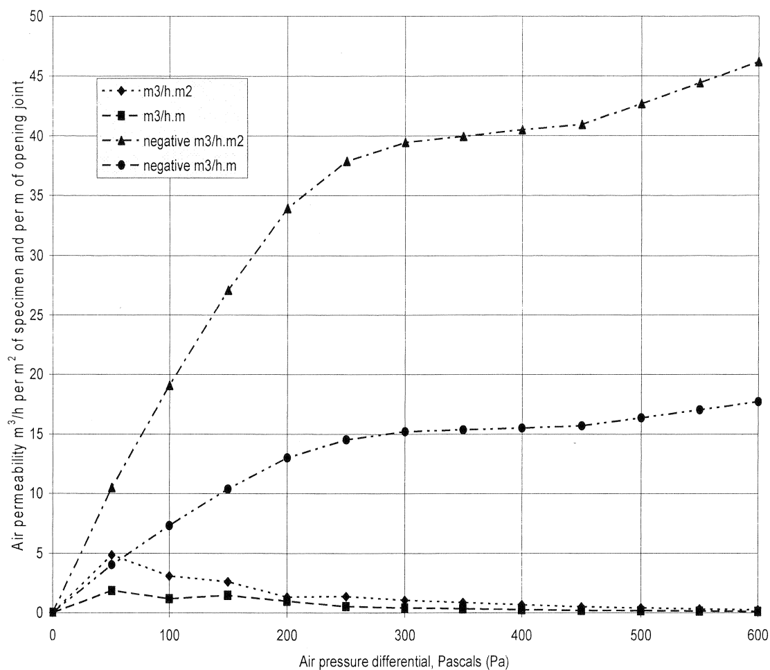
Figure A1. Air permeability under positive and negative air pressure; test results
